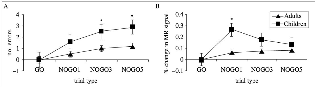
Figure 3 Panel A. Number of errors made on nogo trials as a function of the number of preceding go trials. Panel B. Percent change in MR signal to nogo trials as a function of the number of preceding go trials in regions in ventral prefrontal cortex, right dorsolateral prefrontal cortex, and the right parietal lobe. NOGO1 indicates a nogo trial preceded by 1 go trial; NOGO3 indicates a nogo trial preceded by 3 go trials; NOGO5 indicates a nogo trial preceded by 5 go trials; * indicates p < 0.05 .
